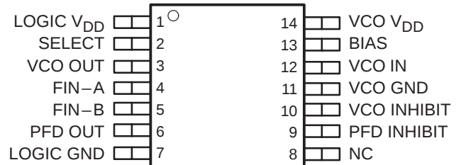
PW PACKAGE † (TOP VIEW)
